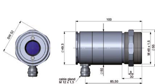
Sensing head
