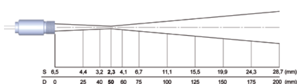
Optics CT LT CF, D:S = 22:1 (far field = 6:1)
