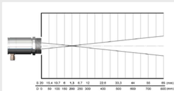
Measurement spot diameter (S) depending on the measurement distance (D) with an IR thermometer
